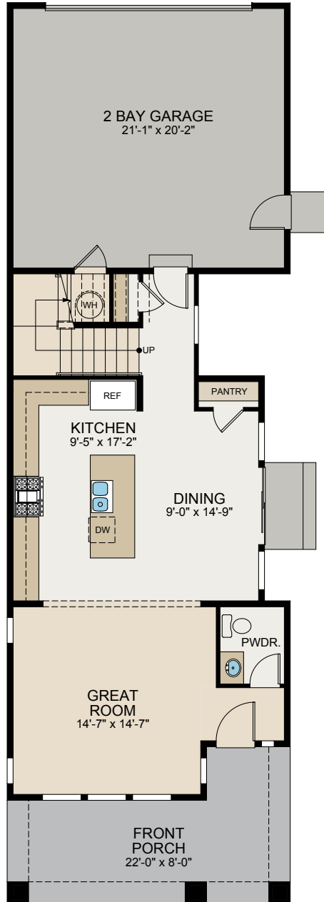
FIRST FLOOR
